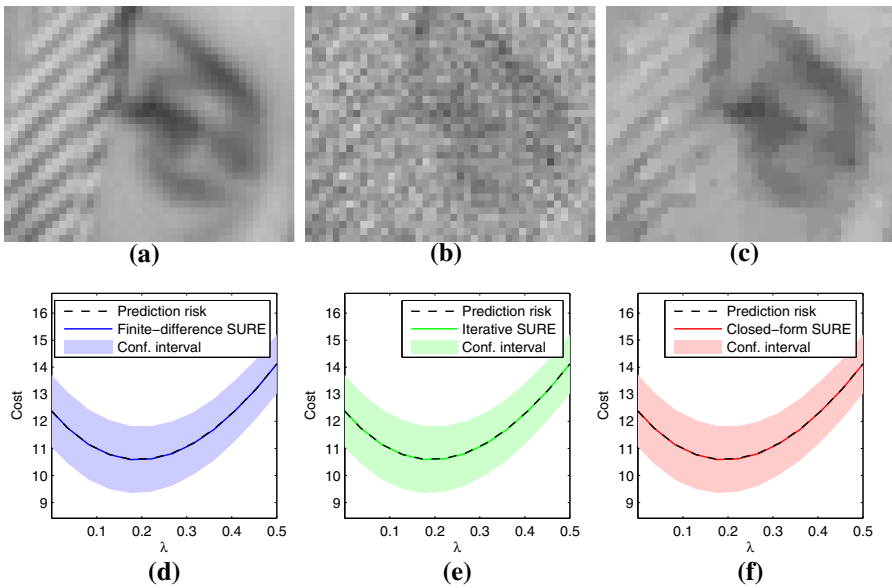
Fig. 2 a Original image \beta_0 . b Least squares estimate X^+y . c \widehat{\beta}(y) obtained for the value of \lambda minimizing the SURE estimate. d–f Prediction risk, average SURE and its confidence interval ( \pm standard deviation) as a function of \lambda , respectively, for the finite difference approach (Ramani et al. 2008), the iterative approach (Deledalle et al. 2014), and our proposed approach
