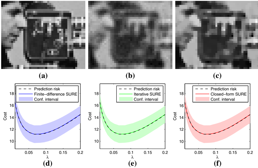
Fig. 1 a Original image \beta_0 . b Blurry observation y . c \widehat{\beta}(y) obtained for the value of \lambda minimizing the SURE estimate. d–f Prediction risk, average SURE and its confidence interval ( \pm standard deviation) as a function of \lambda , respectively, for the finite difference approach (Ramani et al. 2008), the iterative approach (Vonesch et al. 2008), and our proposed approach
