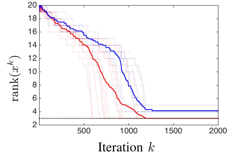
Fig. 2. Evolution of \text{rank}(x^k) as a function of k during the progress of Forward-Backward iterations (13) to solve (1) using observations y = \Phi x_0 + w . The light red (resp. blue) curves represent the evolution for an input x_0 satisfying \mathbf{IC}(x_0) < 1 (resp. \mathbf{IC}(x_0) > 1 ). The bold red (resp. blue) curve is the average of the light red (resp. blue) curves.
