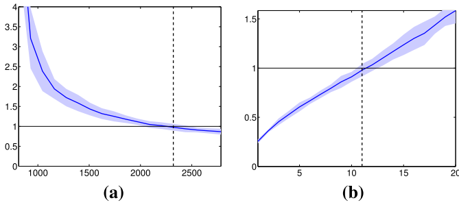
Fig. 1. Curves of \mathbf{IC}(x_0) (central solid line: average, blue shaded band: \pm 3 \times standard deviation) for 25 realizations of \Phi \in \mathbb{R}^{p \times n_0^2} from the standard Gaussian ensemble, where n_0 = 10^3 , and a random x_0 = AB^* of rank r where A, B \in \mathbb{R}^{n_0 \times r} are Gaussian matrices. (a) \mathbf{IC}(x_0) as a function of p for a fixed r = 4 . The vertical dashed line shows the threshold p = r(6n_0 - 5r) indicated by (19). (b) \mathbf{IC}(x_0) as a function of r for a fixed p = 0.6n_0^2 . The vertical dashed line shows the threshold r = (3n_0 - \sqrt{9n_0^2 - 5p})/5 indicated by (19).
